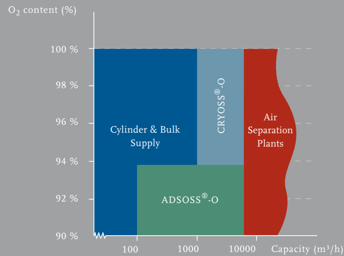
Choice of product line depends on purity, capacity and pressure requirements.
