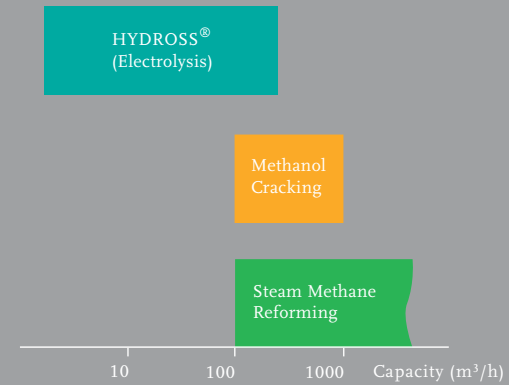
Choice of product line depends on raw material costs and capacity.
